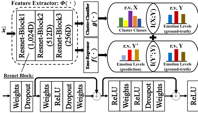
Fig. 1. The process of extracting the DeepMI curriculum metric using the training set. First, the DeepEmoCluster framework is pre-trained, including the feature extractor \Phi(\cdot) , the cluster classifier g(\cdot) , and the emotional regressor f(\cdot) . Then, the emotional label, the recognized cluster and predicted emotional attributes are used to compute joint probabilities. Finally, we derive mutual information measures to estimate the DeepMI metric.
